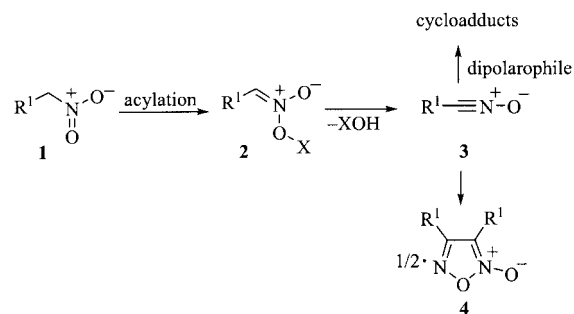
Scheme 1. Dehydration of primary nitro compounds with acylating agents. [a] Ref. [1] [b] Refs. [18,11] [c] Ref. [19] [d] Ref. [20] [e] Refs. [21,22]
